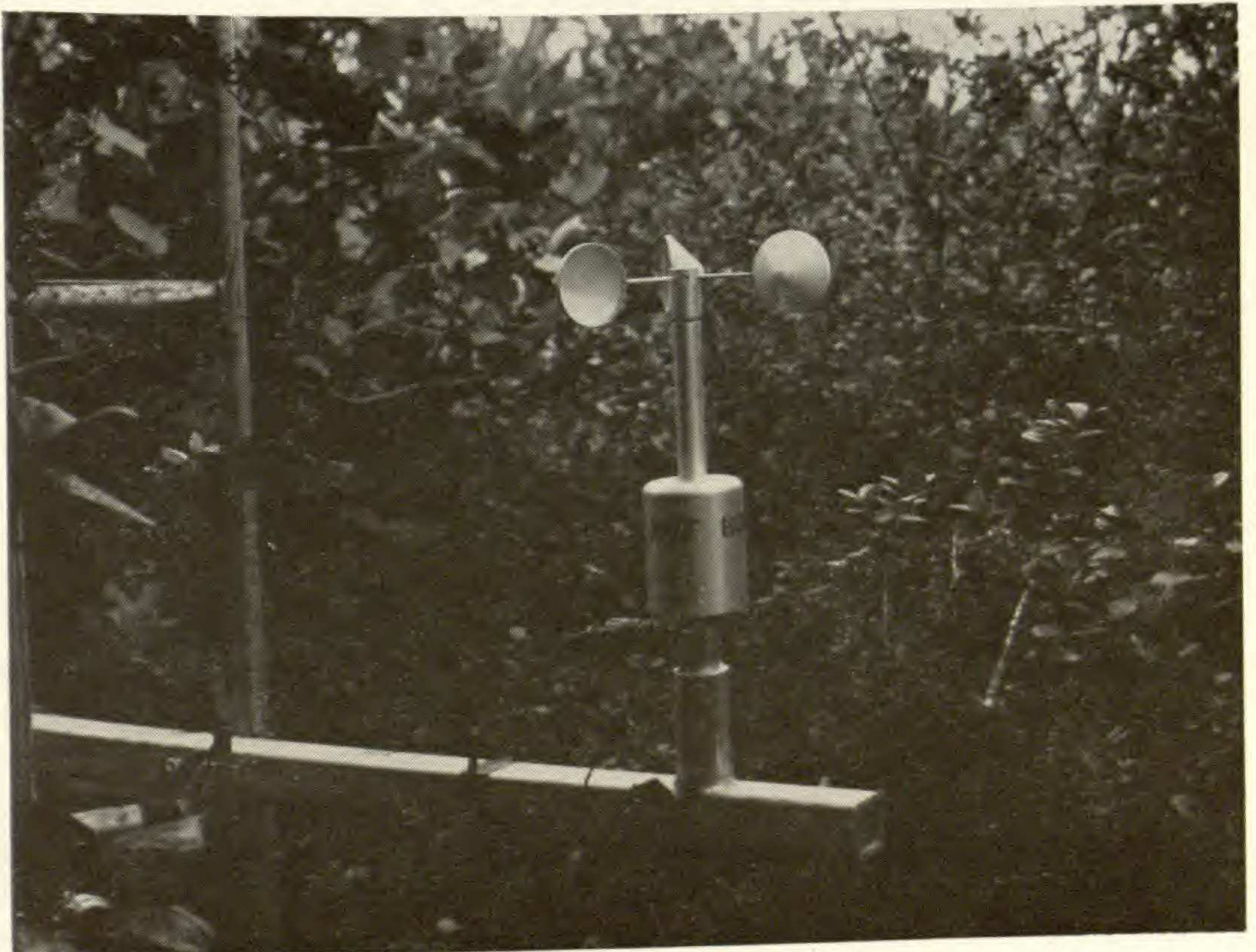
FIG. 7. 3-cup anemometer used for measuring wind speed below the canopy.
